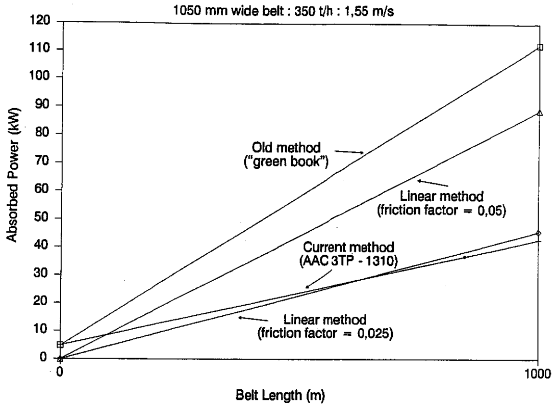
Figure 2: Comparison of Different Design Methods for Conveyors ( 0 – 1000m )
