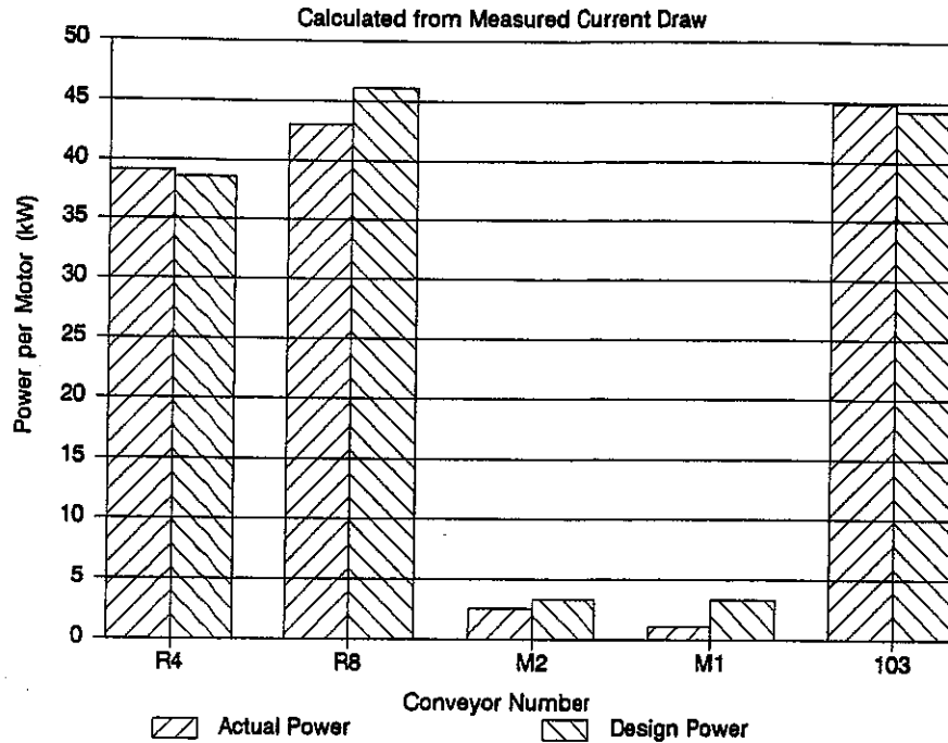
Figure 7: Comparison of Conveyor Powers
