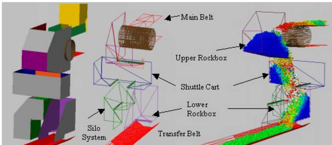
Fig. 6 – Dem boundary surfaces and material flow
