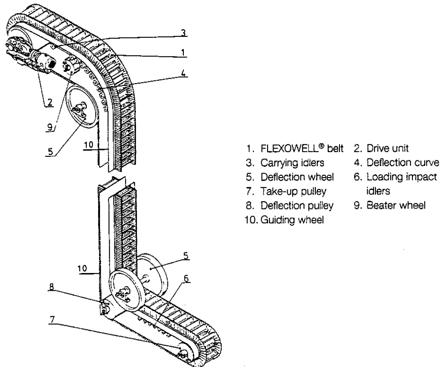
Figure 2. Isometric view of a vertical conveyor [3]
