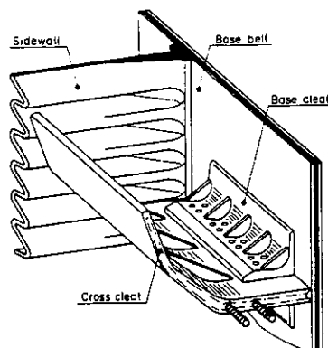
Figure 3. Flexowell belt for vertical conveyor systems [4]
