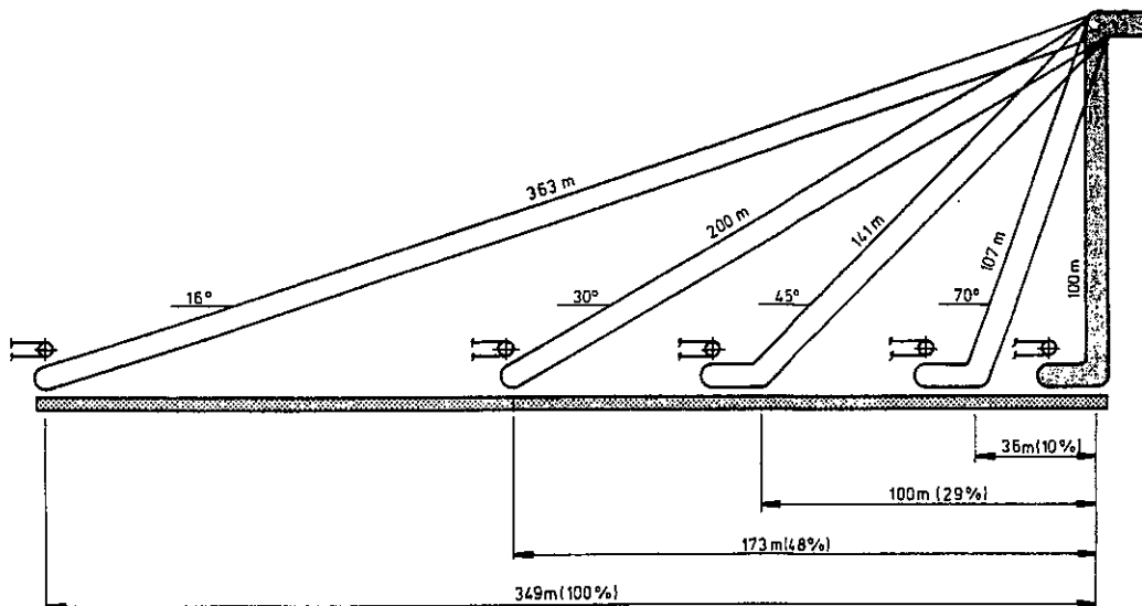
Figure 1. Required length of surface area in relationship to conveyor angle and conveyor height [1]
