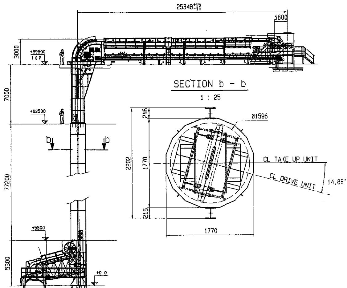
Figure 5. Vertical conveyor for Saldanha Steel/South Africa
