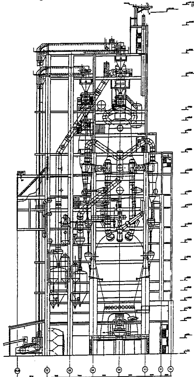
Figure 4. Tower Corex C-2000 with two S-shape Flexotum-systems for Jindal-Steel, India
