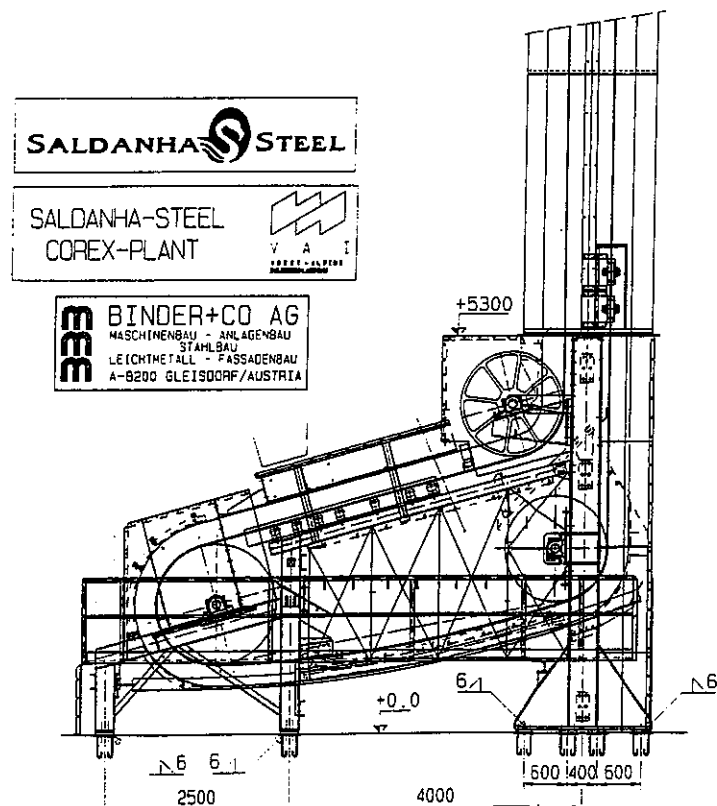
Figure 6. Bottom station of the vertical conveyor
