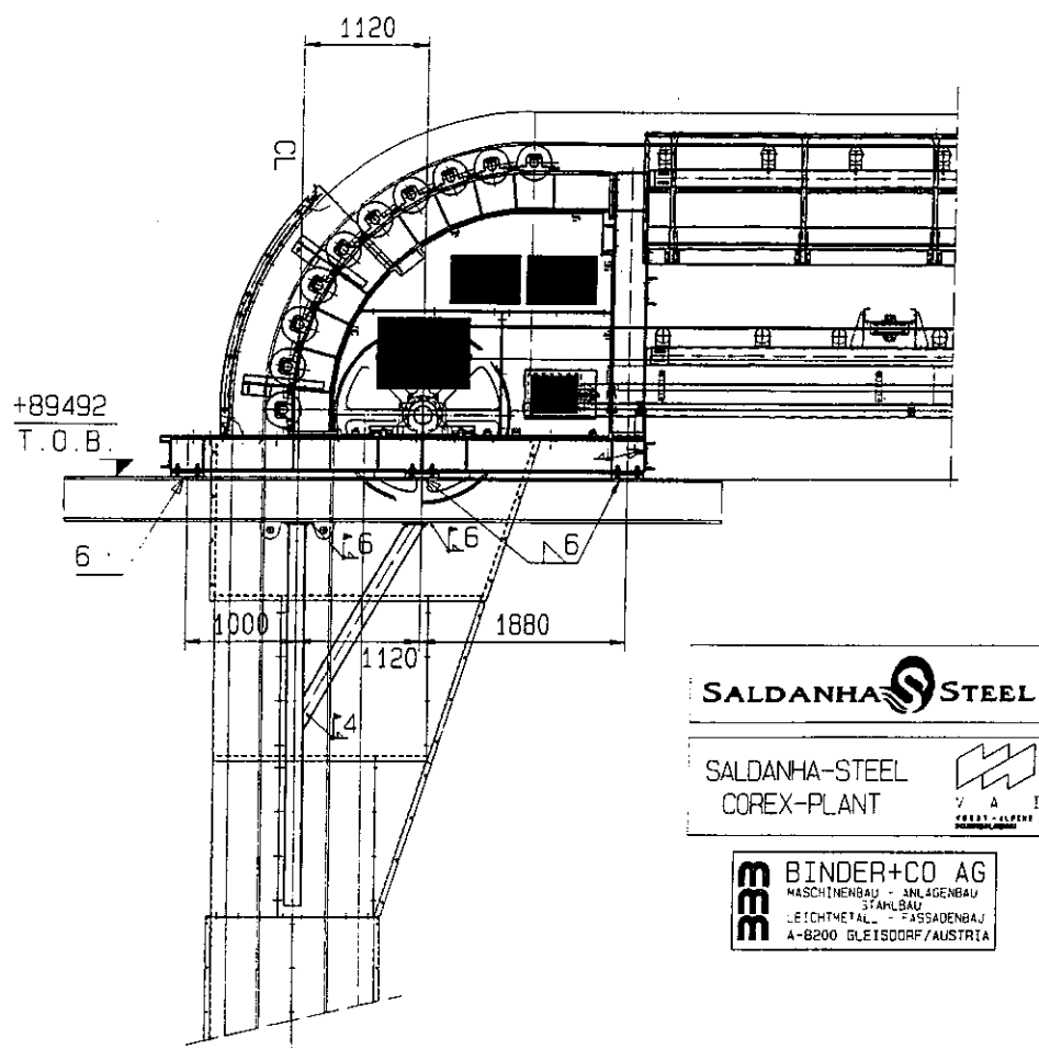
Figure 7. Top deflection unit of the vertical conveyor
